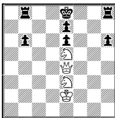
#4 (4+7)
