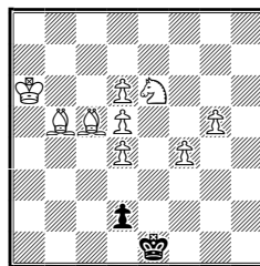
h#3 (9+2) twins
