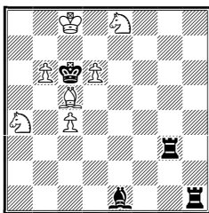
#4 (7+4)
